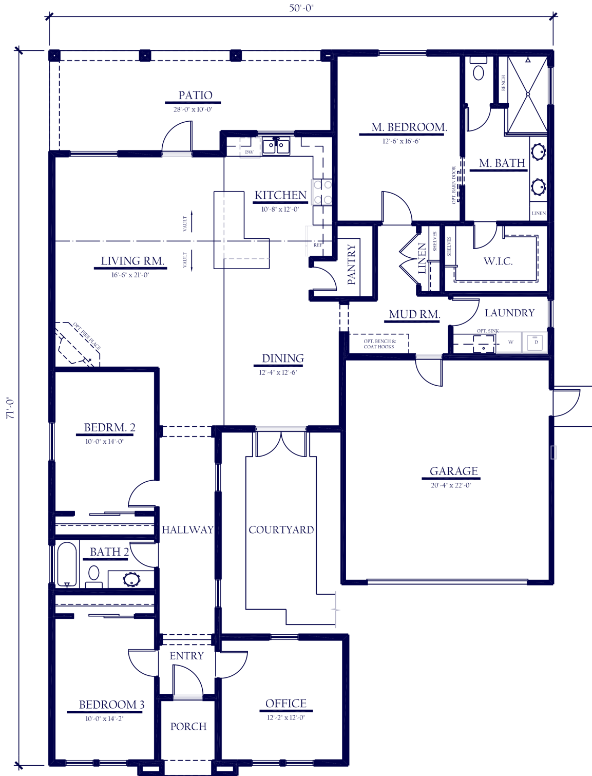
FLOOR PLAN 2177
