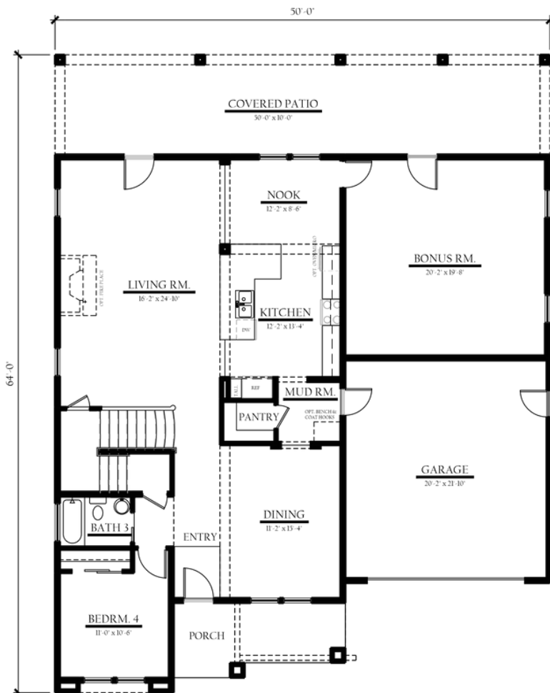
2887 Lower Floorplan
